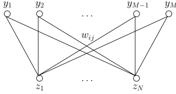
Fig. 2. A bipartite neural network
